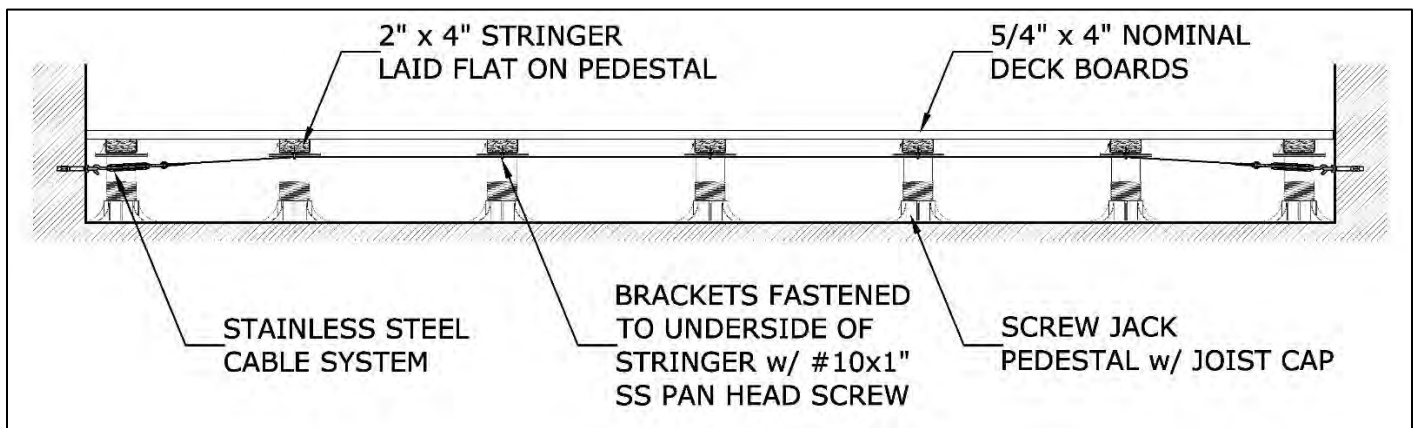
Cable Runs Perpindicular To Stringers And Attaches To Parapet Anchors Using Turn Buckles or Cable Clamps
