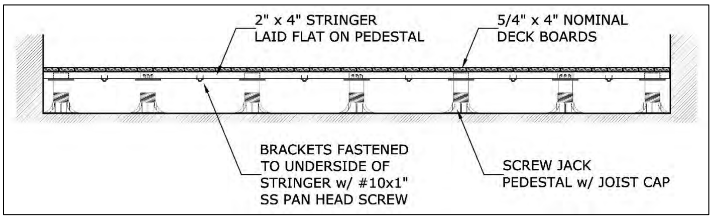
U Brackets Installed Parrallel To Stringers
